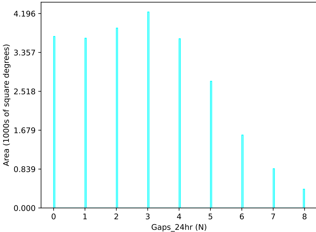
too_elab_r8_d2_giz_v3.4_10yrs u band: Gaps_24hr
