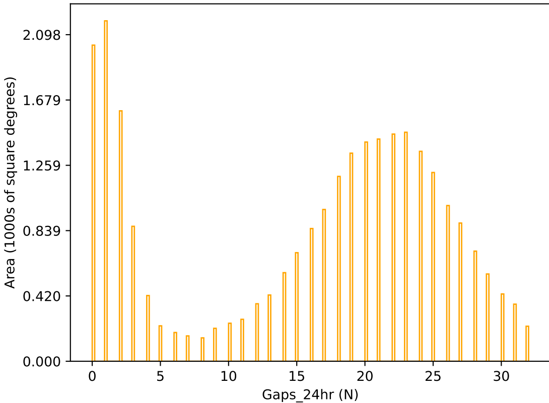
too_elab_r8_d2_giz_v3.4_10yrs r band: Gaps_24hr
