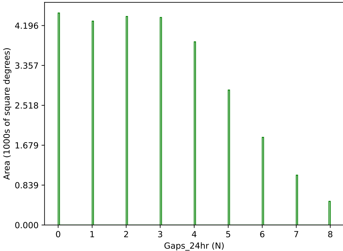
too_elab_r8_d2_giz_v3.4_10yrs g band: Gaps_24hr
