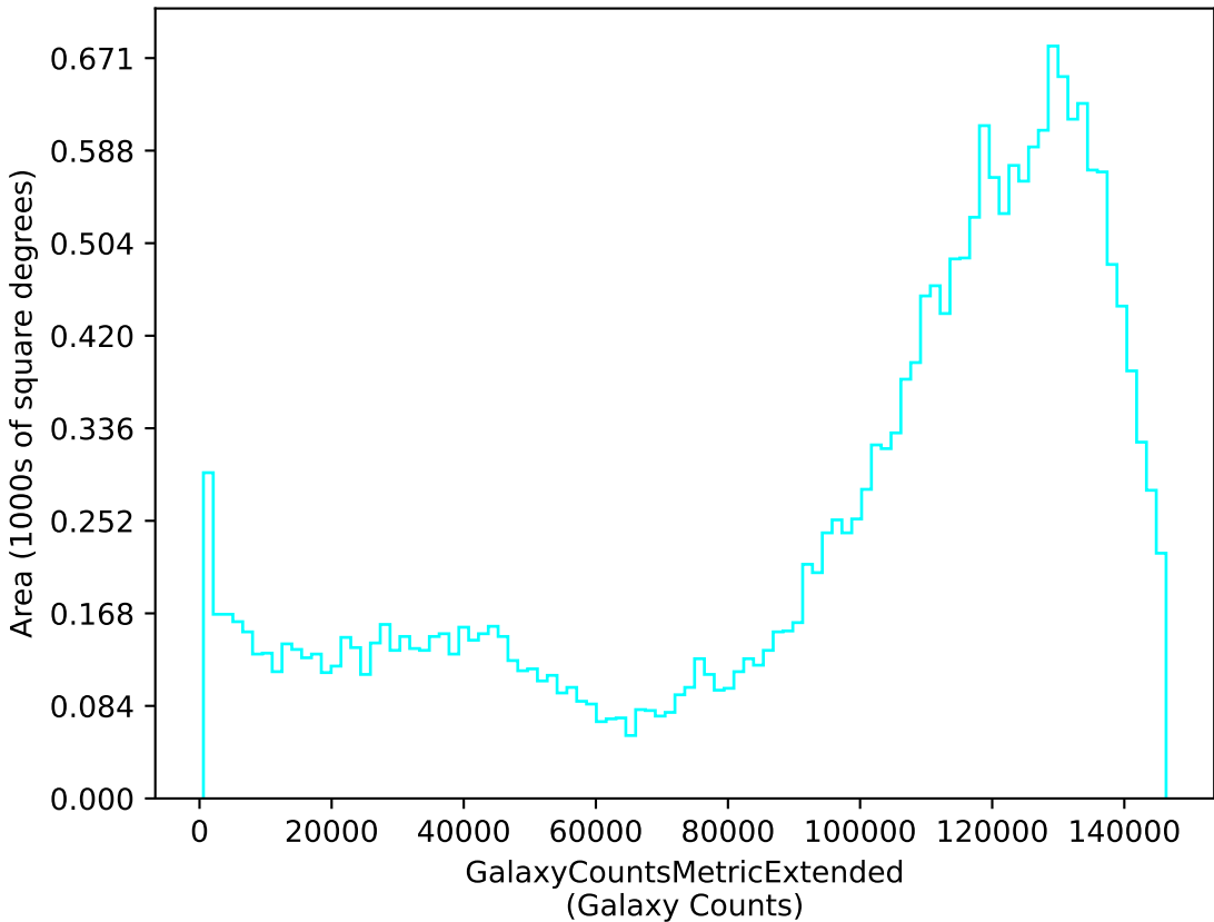
too_elab_r8_d2_giz_v3.4_10yrs u: GalaxyCountsMetricExtended
