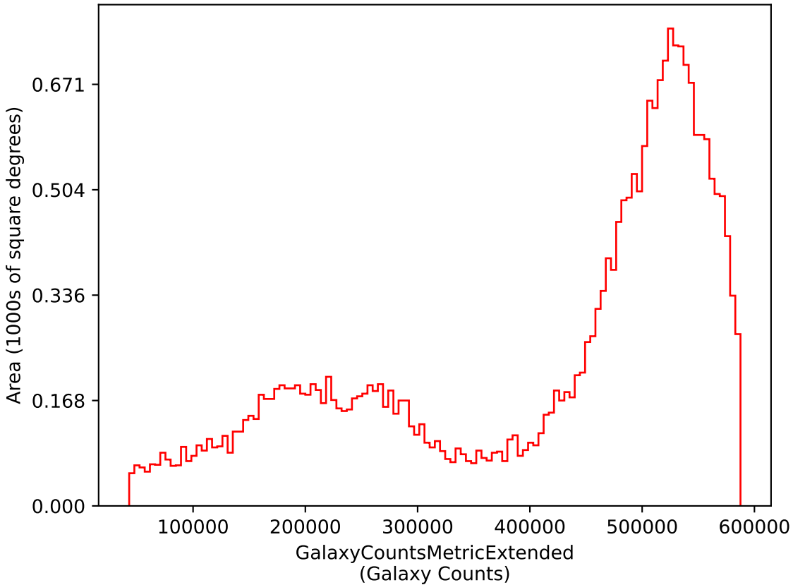
too_elab_r8_d2_giz_v3.4_10yrs i: GalaxyCountsMetricExtended
