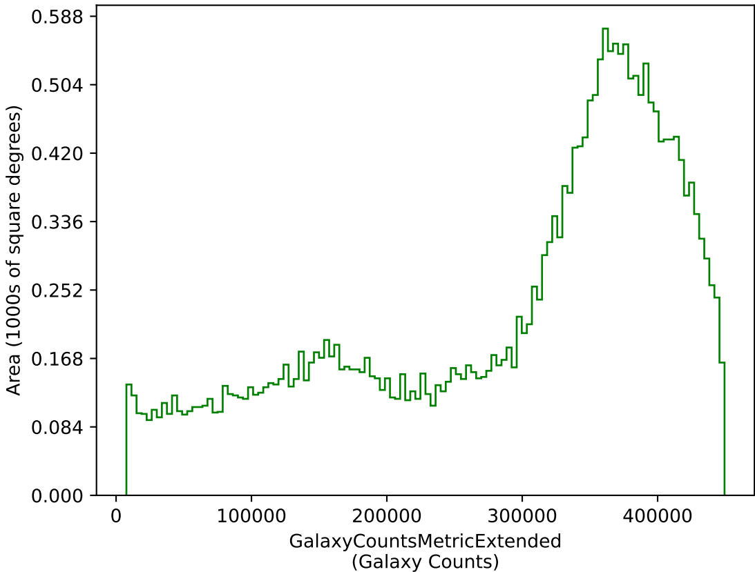
too_elab_r8_d2_giz_v3.4_10yrs g: GalaxyCountsMetricExtended
