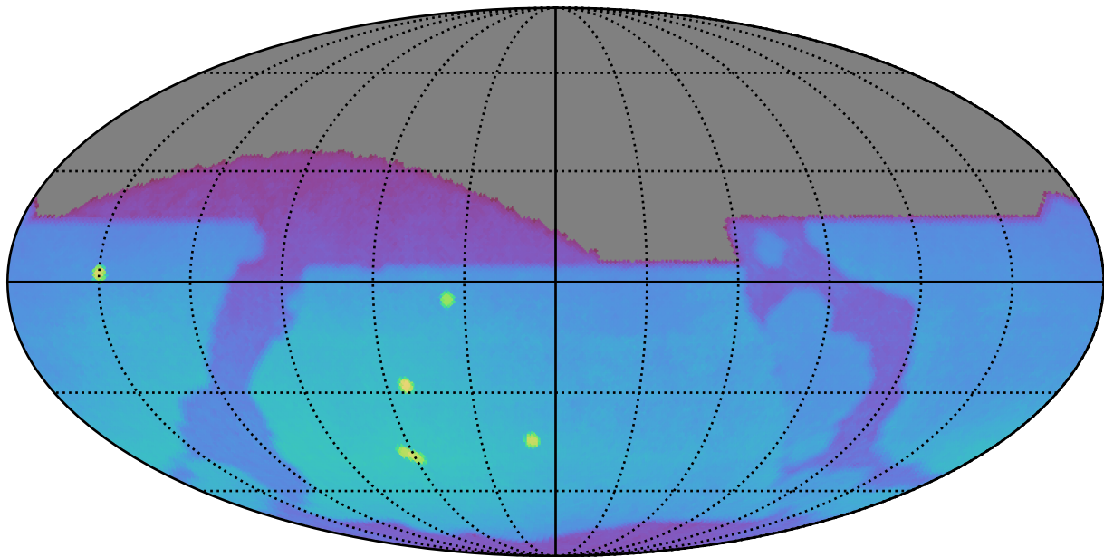
too_elab_r8_d2_giz_v3.4_10yrs : Brown Dwarf, L7
