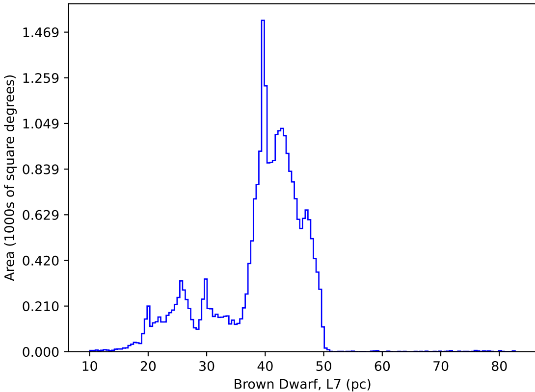
too_elab_r8_d2_giz_v3.4_10yrs : Brown Dwarf, L7
