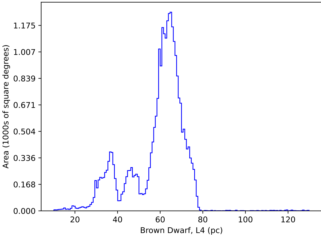
too_elab_r8_d2_giz_v3.4_10yrs : Brown Dwarf, L4
