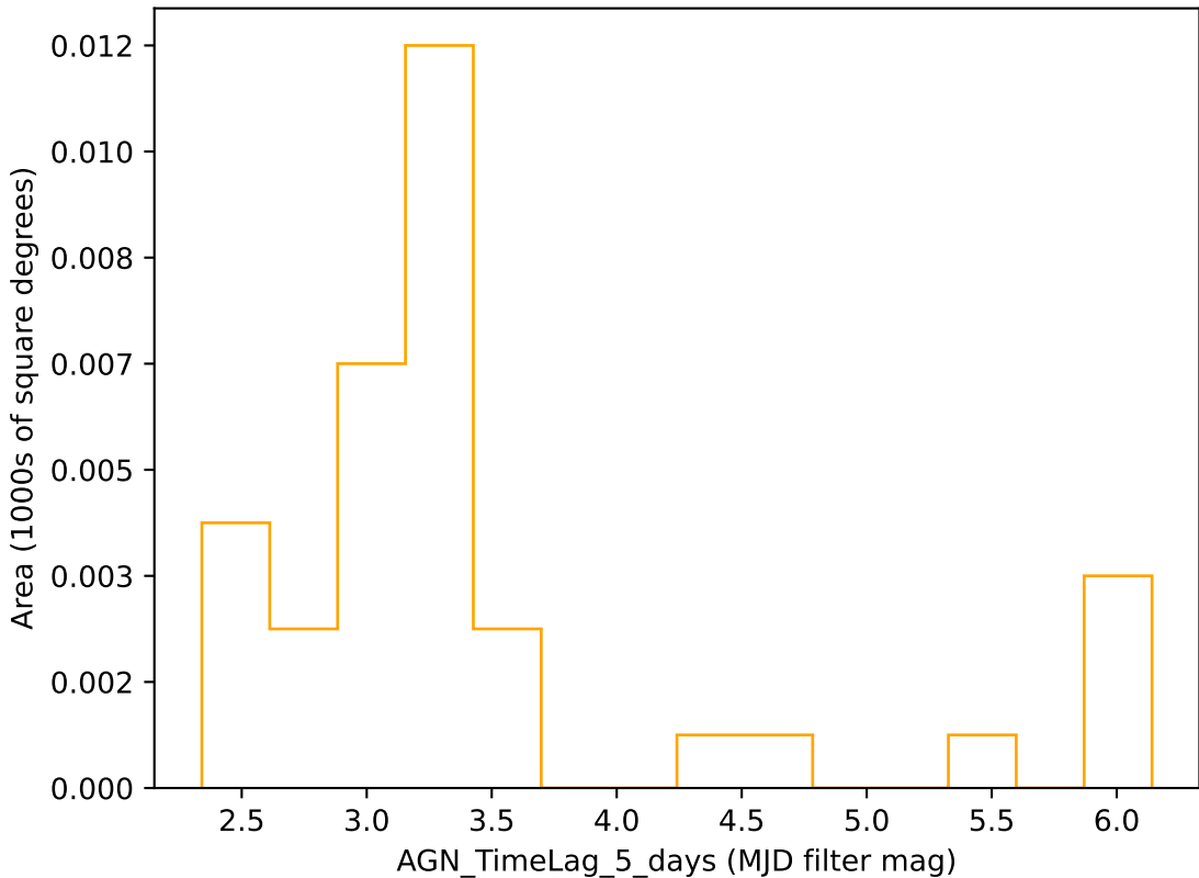
too_elab_r8_d2_giz_v3.4_10yrs r band: AGN_TimeLag_5_days
