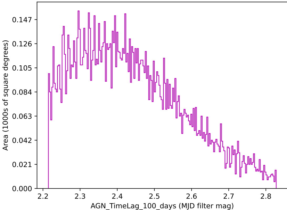
too_elab_r8_d2_giz_v3.4_10yrs z band: AGN_TimeLag_100_days
