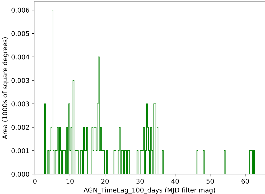
too_elab_r8_d2_giz_v3.4_10yrs g band: AGN_TimeLag_100_days
