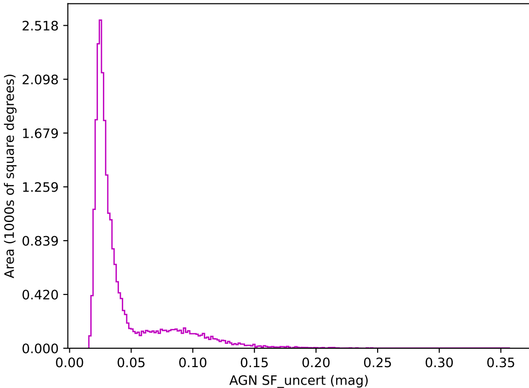
too_elab_r8_d2_giz_v3.4_10yrs z band: AGN SF_uncert
