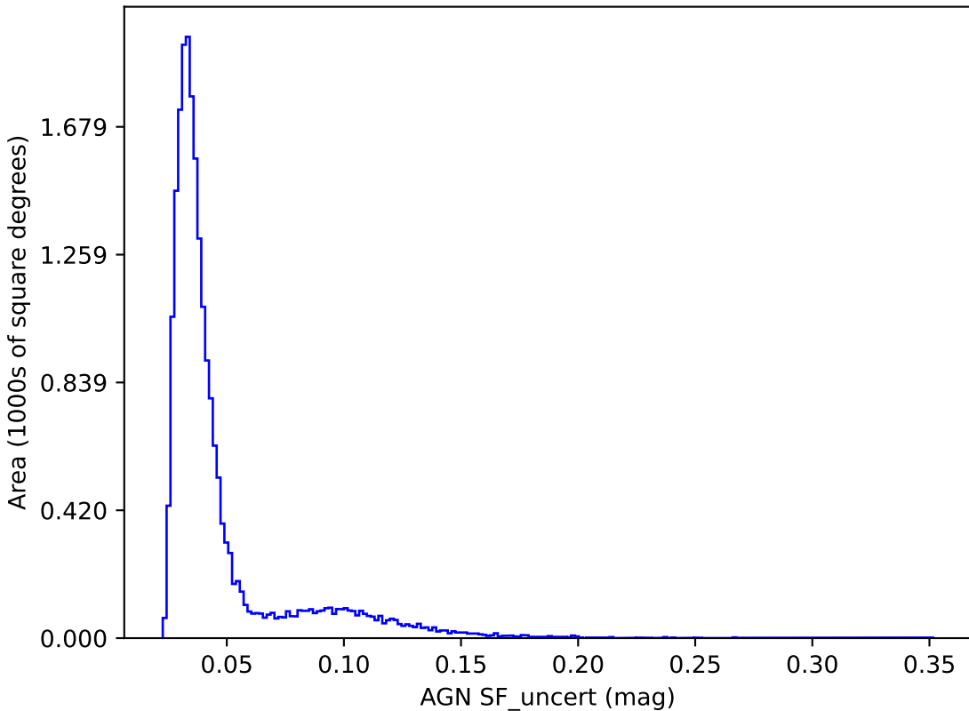
too_elab_r8_d2_giz_v3.4_10yrs y band: AGN SF_uncert
