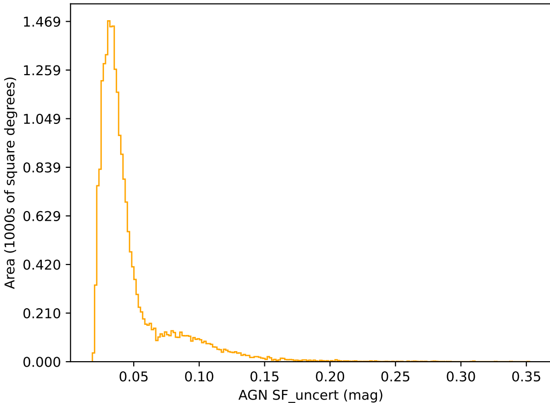
too_elab_r8_d2_giz_v3.4_10yrs r band: AGN SF_uncert
