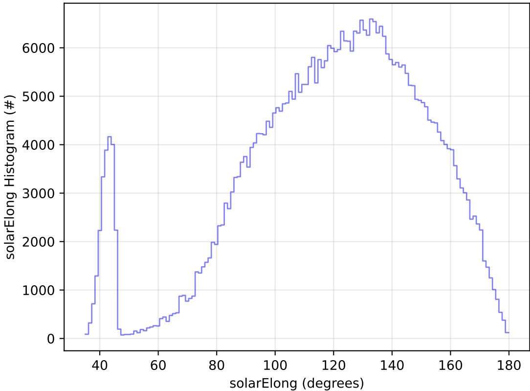
too_elab_r8_d2_giz_v3.4_10yrs WFD z band: solarElong Histogram
