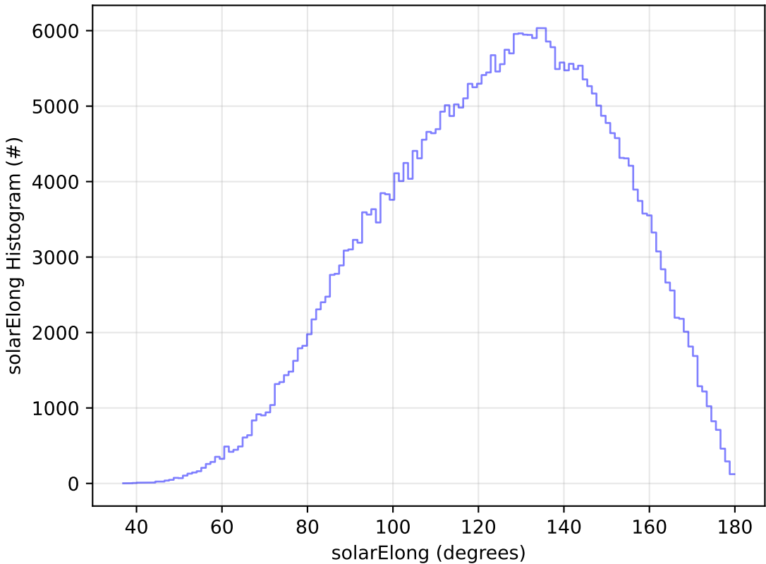
too_elab_r8_d2_giz_v3.4_10yrs WFD y band: solarElong Histogram
