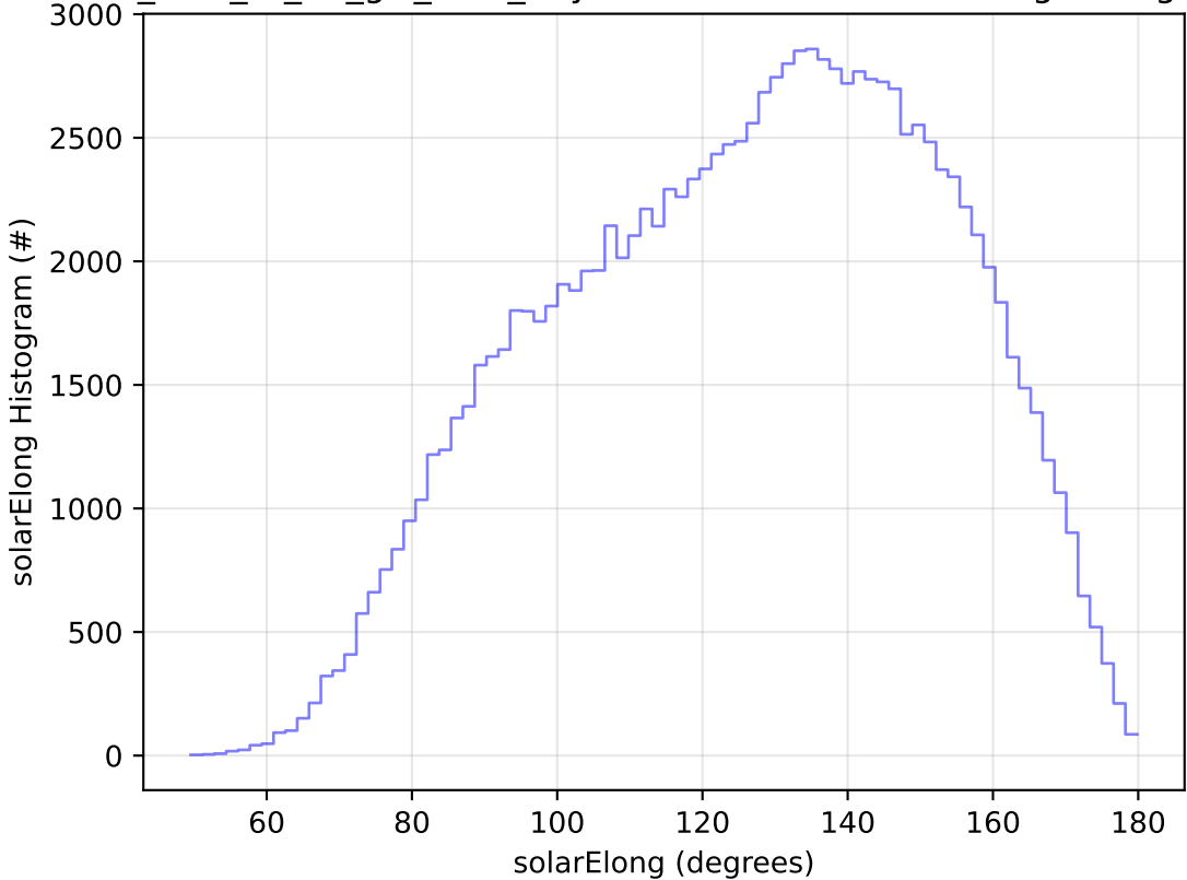
too_elab_r8_d2_giz_v3.4_10yrs WFD u band: solarElong Histogram
