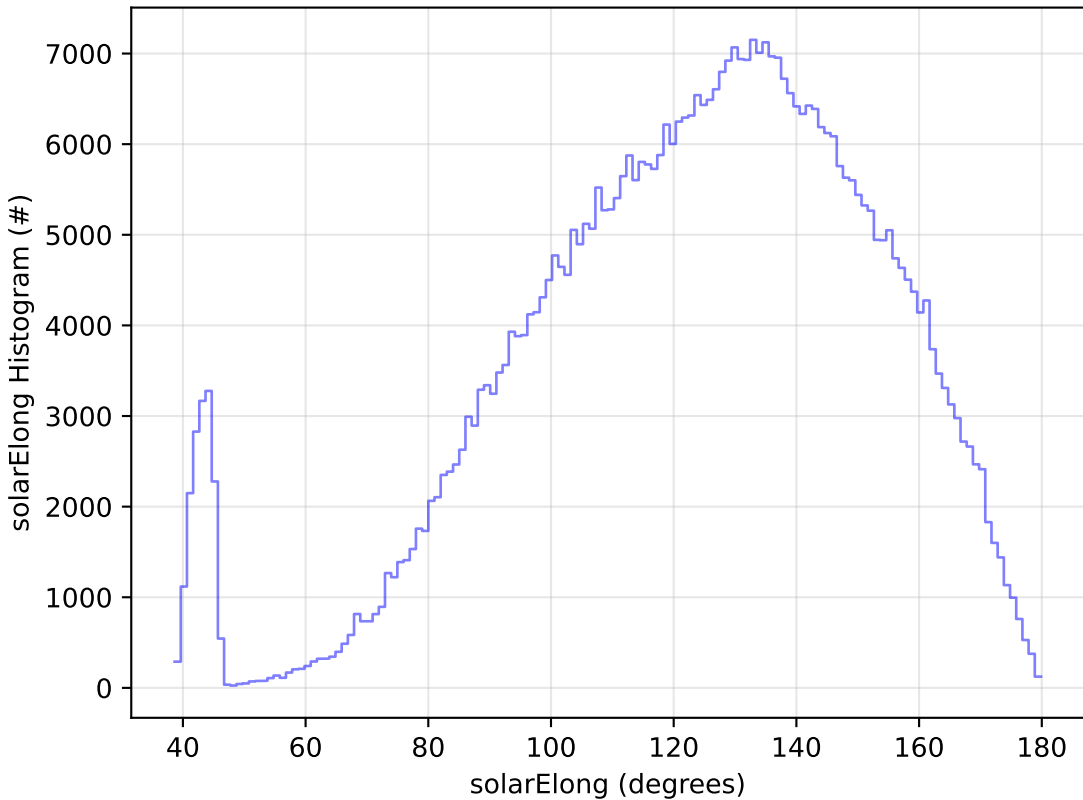
too_elab_r8_d2_giz_v3.4_10yrs WFD r band: solarElong Histogram
