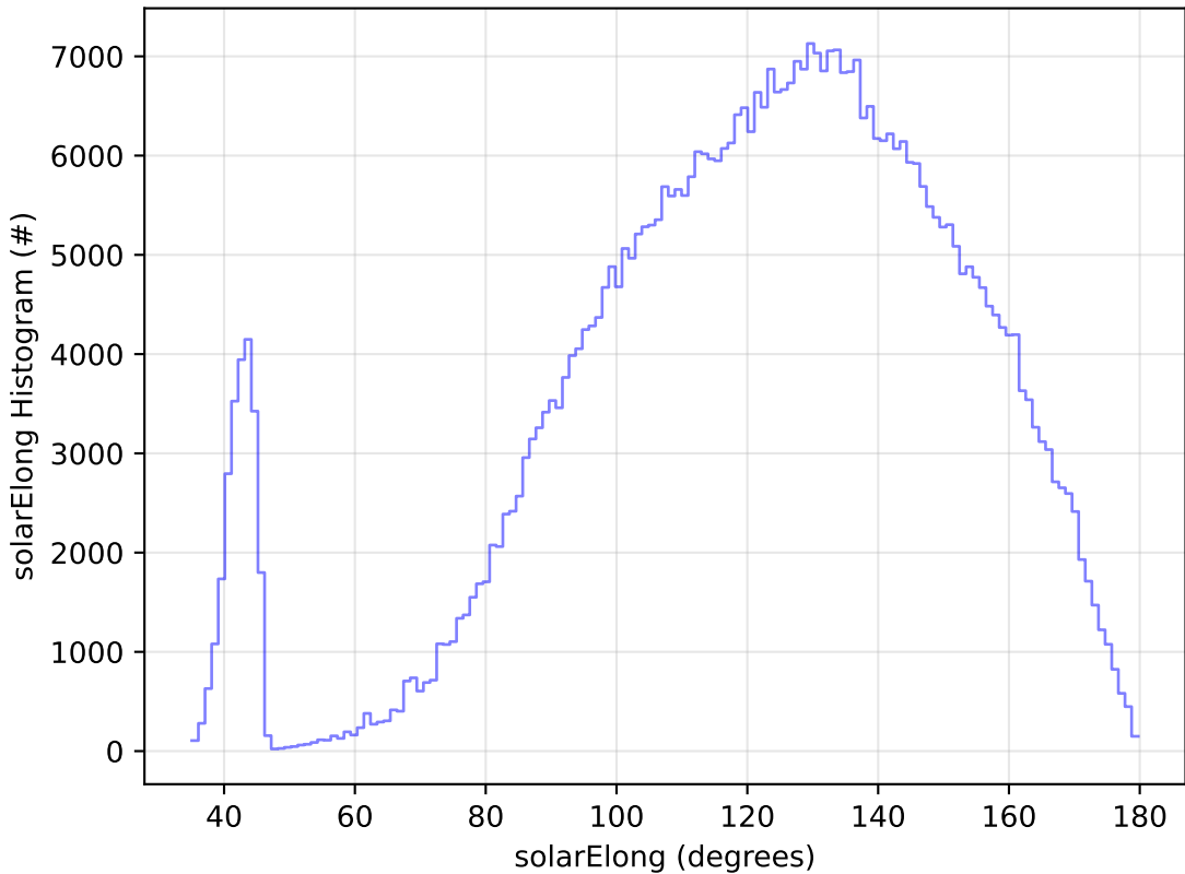
too_elab_r8_d2_giz_v3.4_10yrs WFD i band: solarElong Histogram
