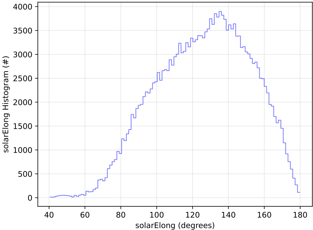
too_elab_r8_d2_giz_v3.4_10yrs WFD g band: solarElong Histogram
