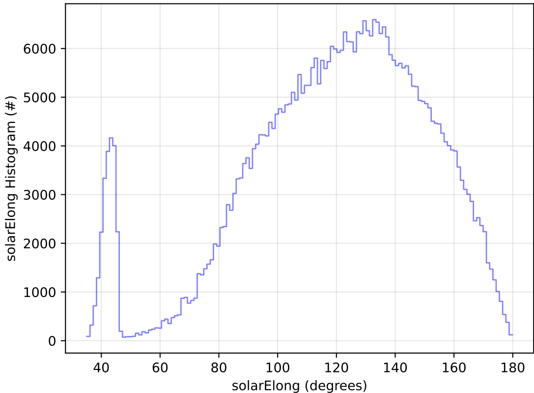
too_elab_r8_d2_giz_v3.4_10yrs All sky z band: solarElong Histogram
