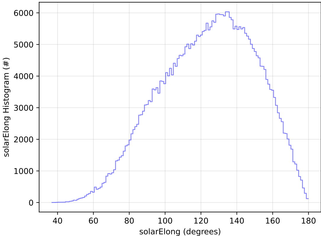
too_elab_r8_d2_giz_v3.4_10yrs All sky y band: solarElong Histogram
