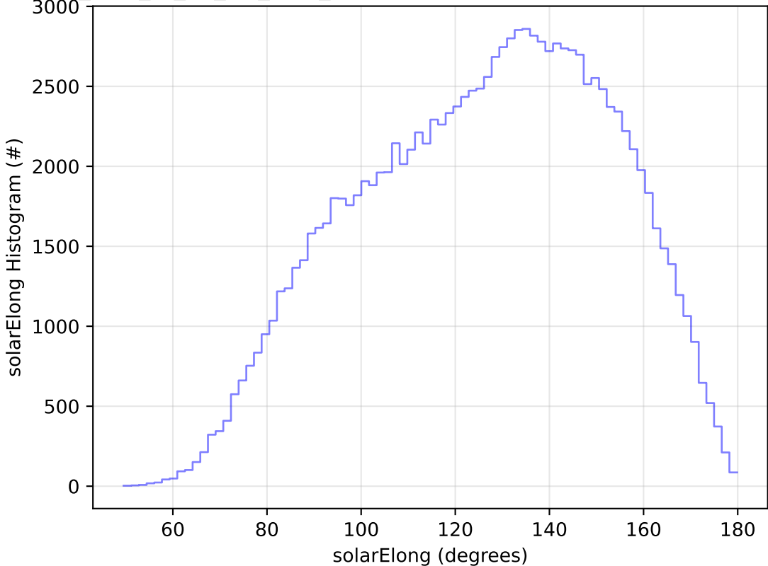
too_elab_r8_d2_giz_v3.4_10yrs All sky u band: solarElong Histogram
