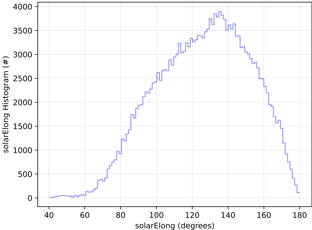
too_elab_r8_d2_giz_v3.4_10yrs All sky g band: solarElong Histogram
