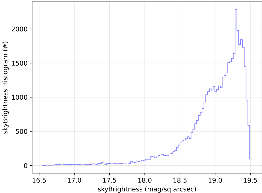
too_elab_r8_d2_giz_v3.4_10yrs Yr 1 z band: skyBrightness Histogram
