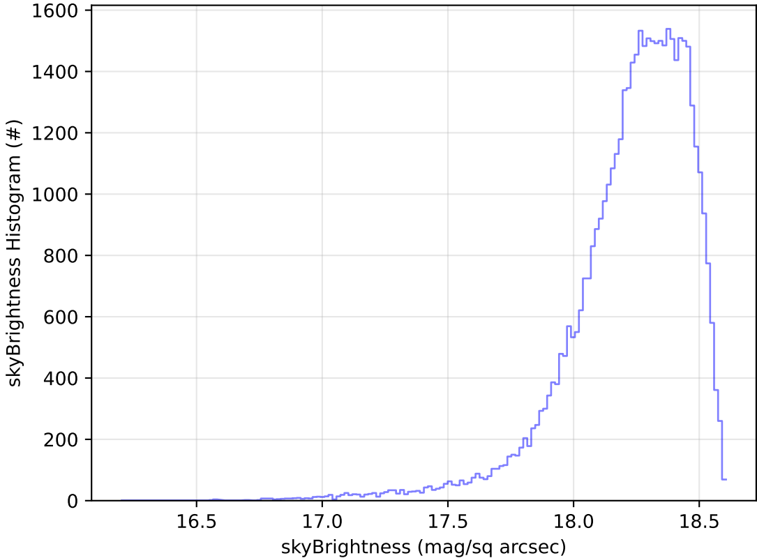
too_elab_r8_d2_giz_v3.4_10yrs Yr 1 y band: skyBrightness Histogram
