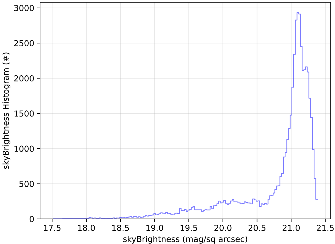
too_elab_r8_d2_giz_v3.4_10yrs Yr 1 r band: skyBrightness Histogram
