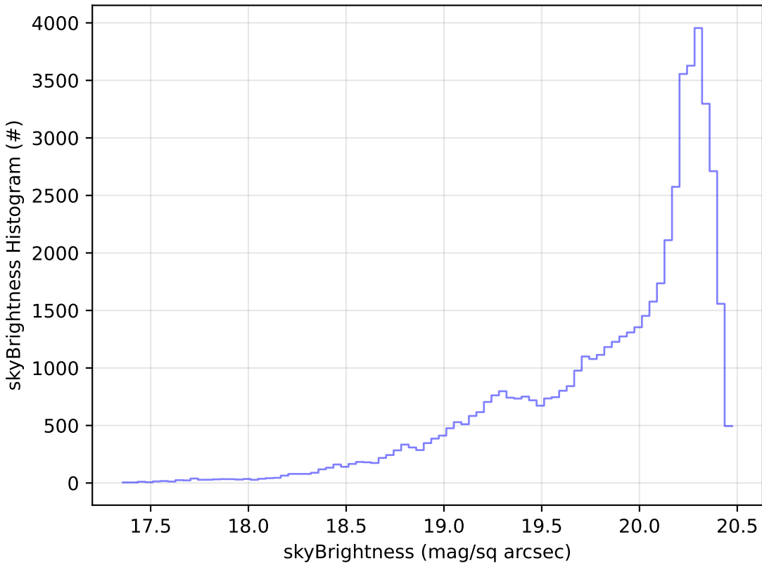
too_elab_r8_d2_giz_v3.4_10yrs Yr 1 i band: skyBrightness Histogram
