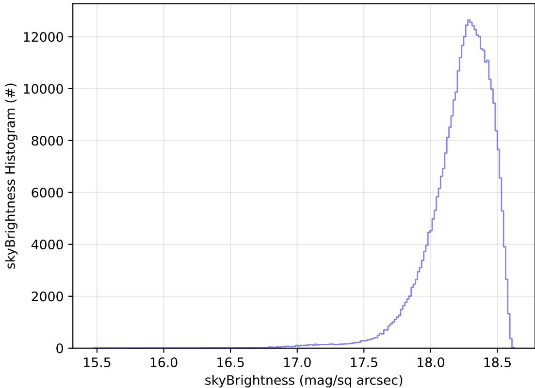
too_elab_r8_d2_giz_v3.4_10yrs WFD y band: skyBrightness Histogram
