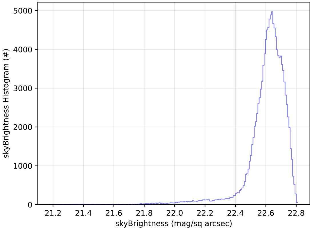
too_elab_r8_d2_giz_v3.4_10yrs WFD u band: skyBrightness Histogram
