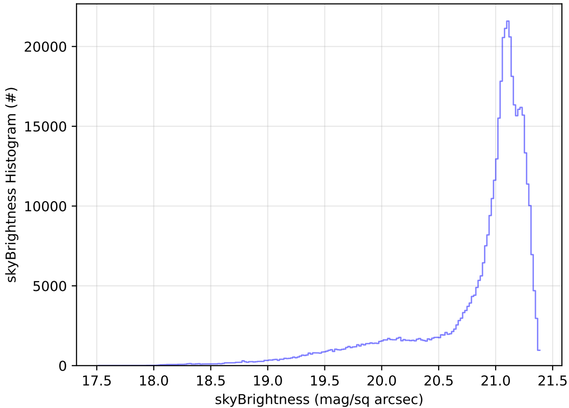
too_elab_r8_d2_giz_v3.4_10yrs WFD r band: skyBrightness Histogram
