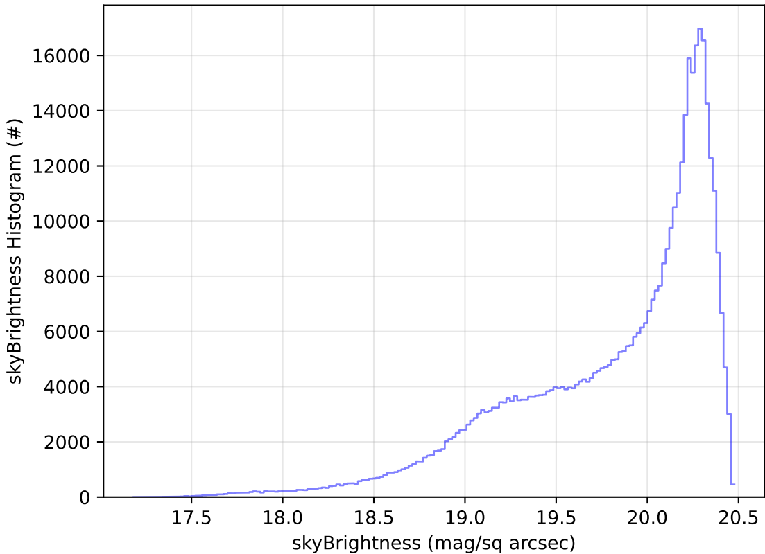
too_elab_r8_d2_giz_v3.4_10yrs WFD i band: skyBrightness Histogram
