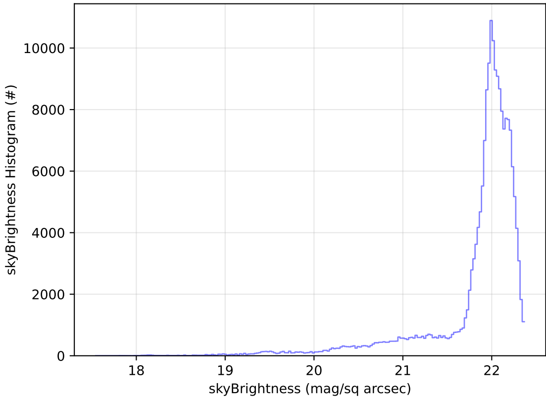
too_elab_r8_d2_giz_v3.4_10yrs WFD g band: skyBrightness Histogram
