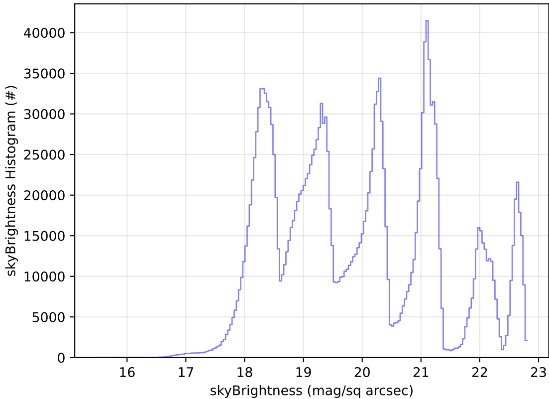
too_elab_r8_d2_giz_v3.4_10yrs WFD all bands: skyBrightness Histogram
