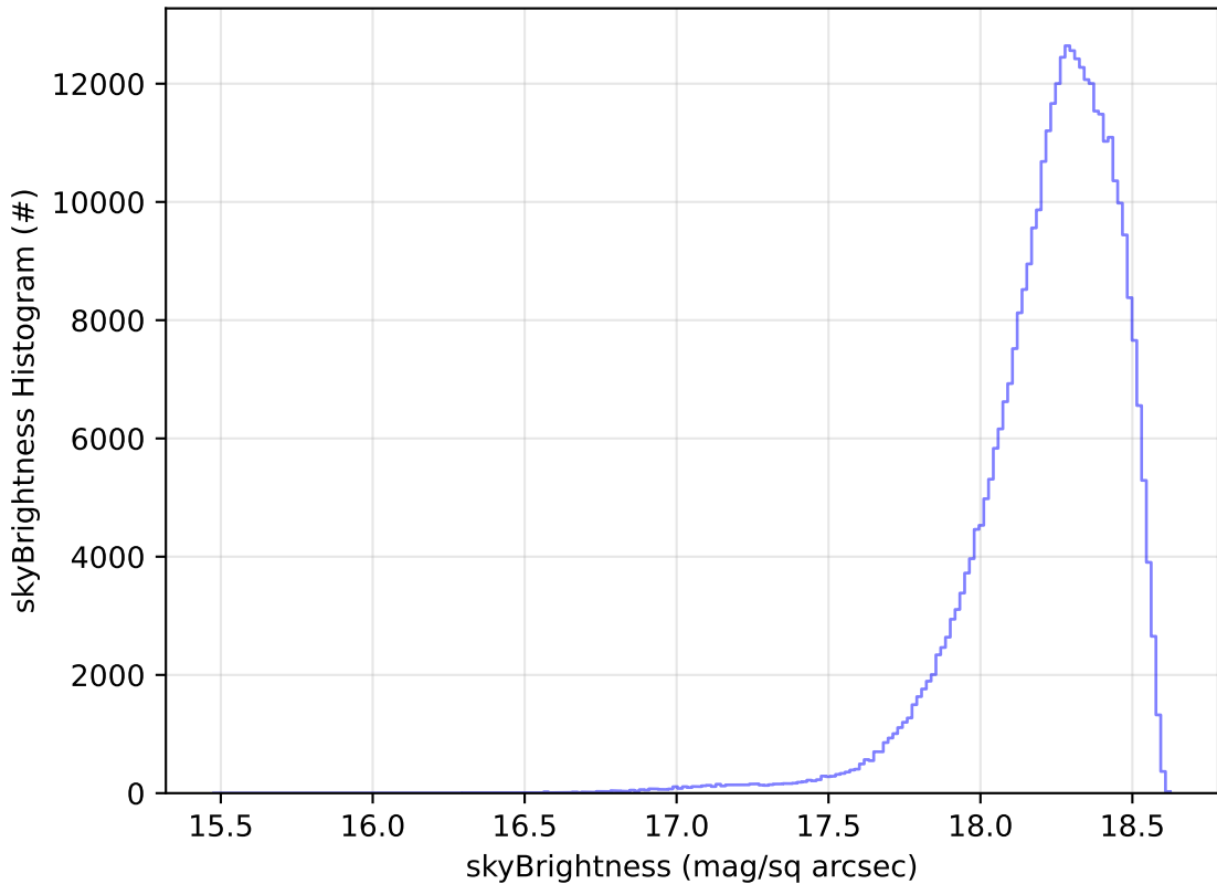
too_elab_r8_d2_giz_v3.4_10yrs All sky y band: skyBrightness Histogram
