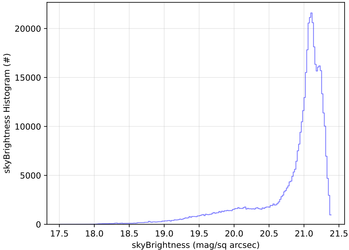
too_elab_r8_d2_giz_v3.4_10yrs All sky r band: skyBrightness Histogram
