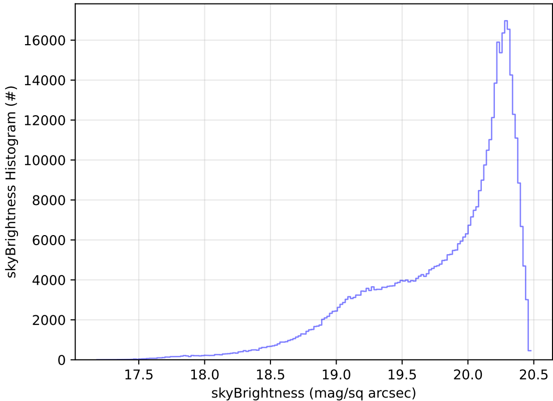
too_elab_r8_d2_giz_v3.4_10yrs All sky i band: skyBrightness Histogram
