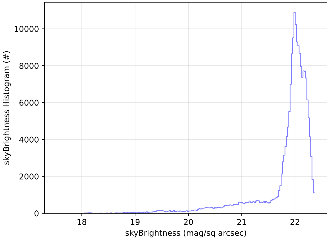
too_elab_r8_d2_giz_v3.4_10yrs All sky g band: skyBrightness Histogram
