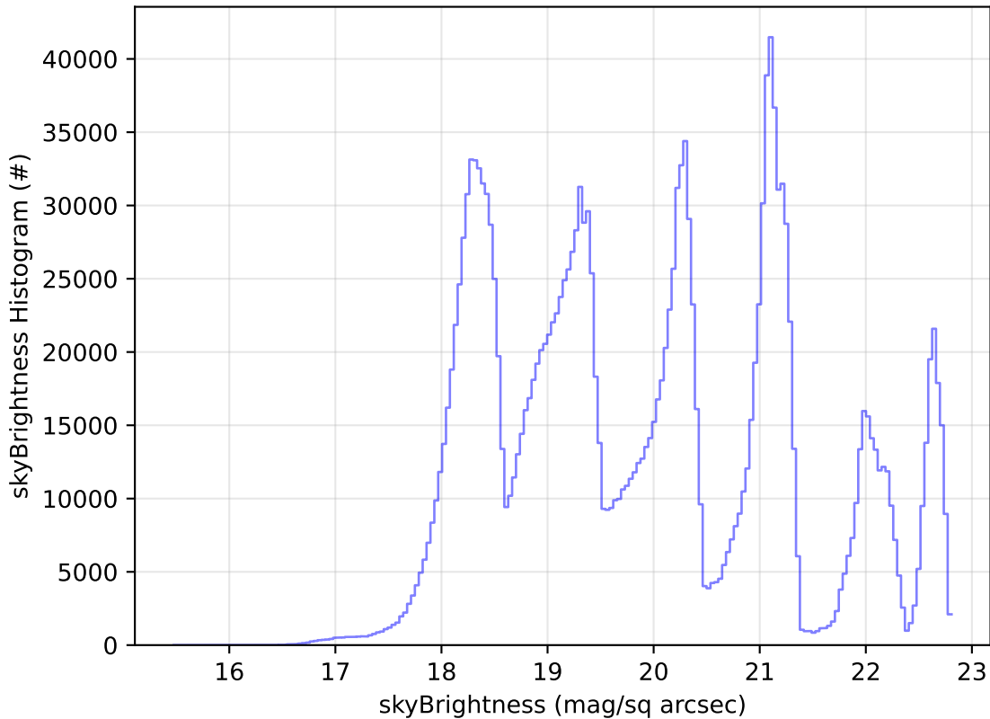
too_elab_r8_d2_giz_v3.4_10yrs All sky all bands: skyBrightness Histogram
