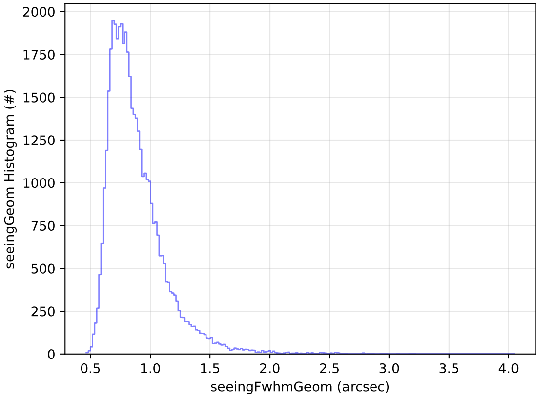
too_elab_r8_d2_giz_v3.4_10yrs Yr 1 z band: seeingGeom Histogram
