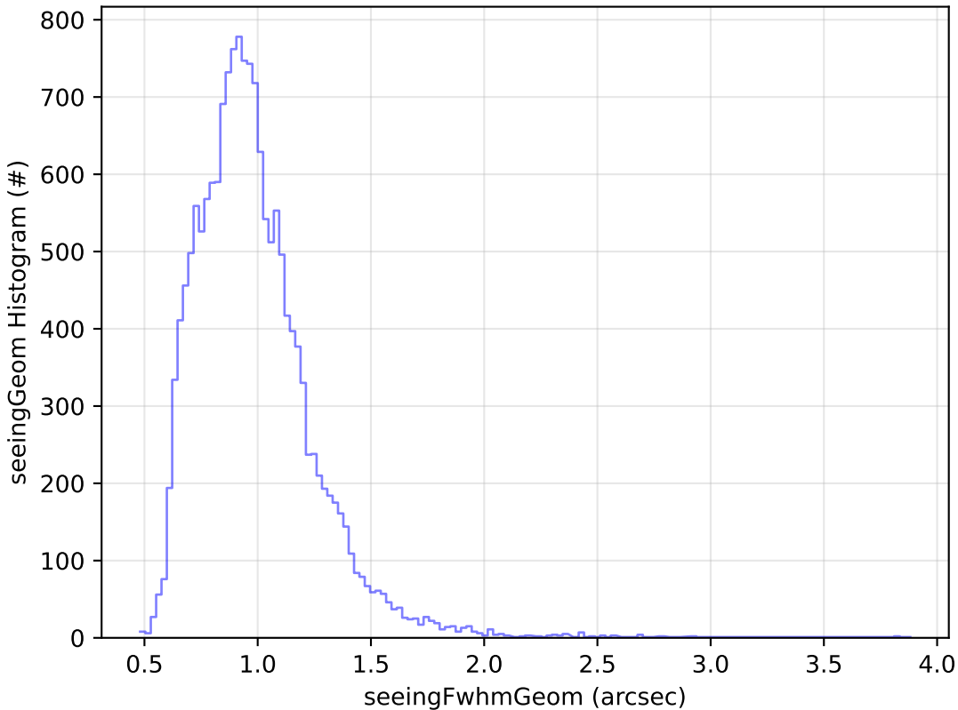
too_elab_r8_d2_giz_v3.4_10yrs Yr 1 u band: seeingGeom Histogram
