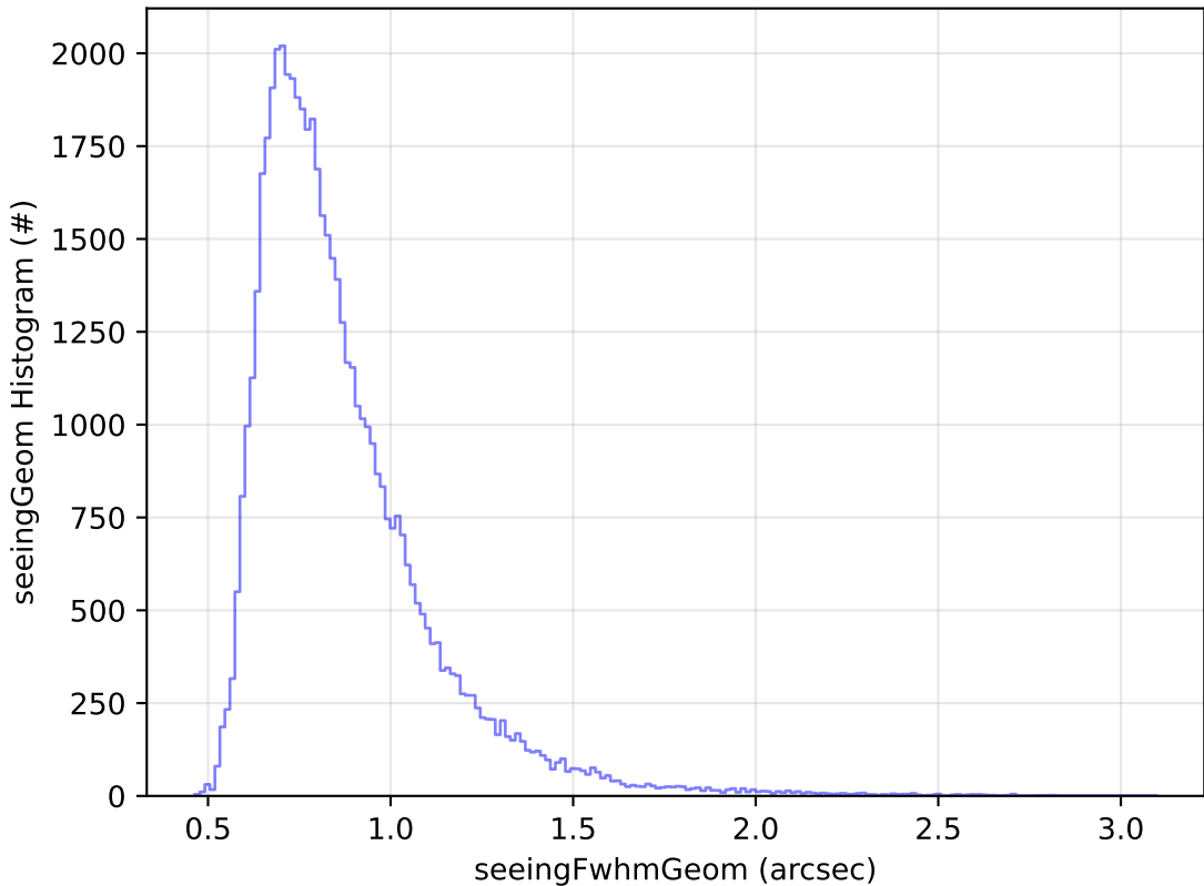
too_elab_r8_d2_giz_v3.4_10yrs Yr 1 i band: seeingGeom Histogram
