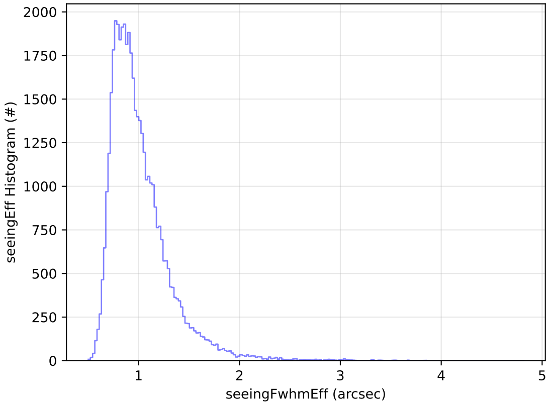
too_elab_r8_d2_giz_v3.4_10yrs Yr 1 z band: seeingEff Histogram
