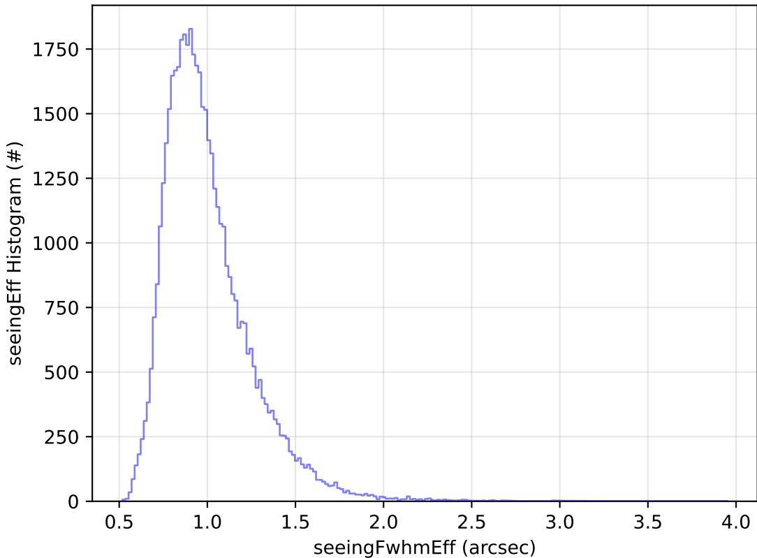
too_elab_r8_d2_giz_v3.4_10yrs Yr 1 y band: seeingEff Histogram
