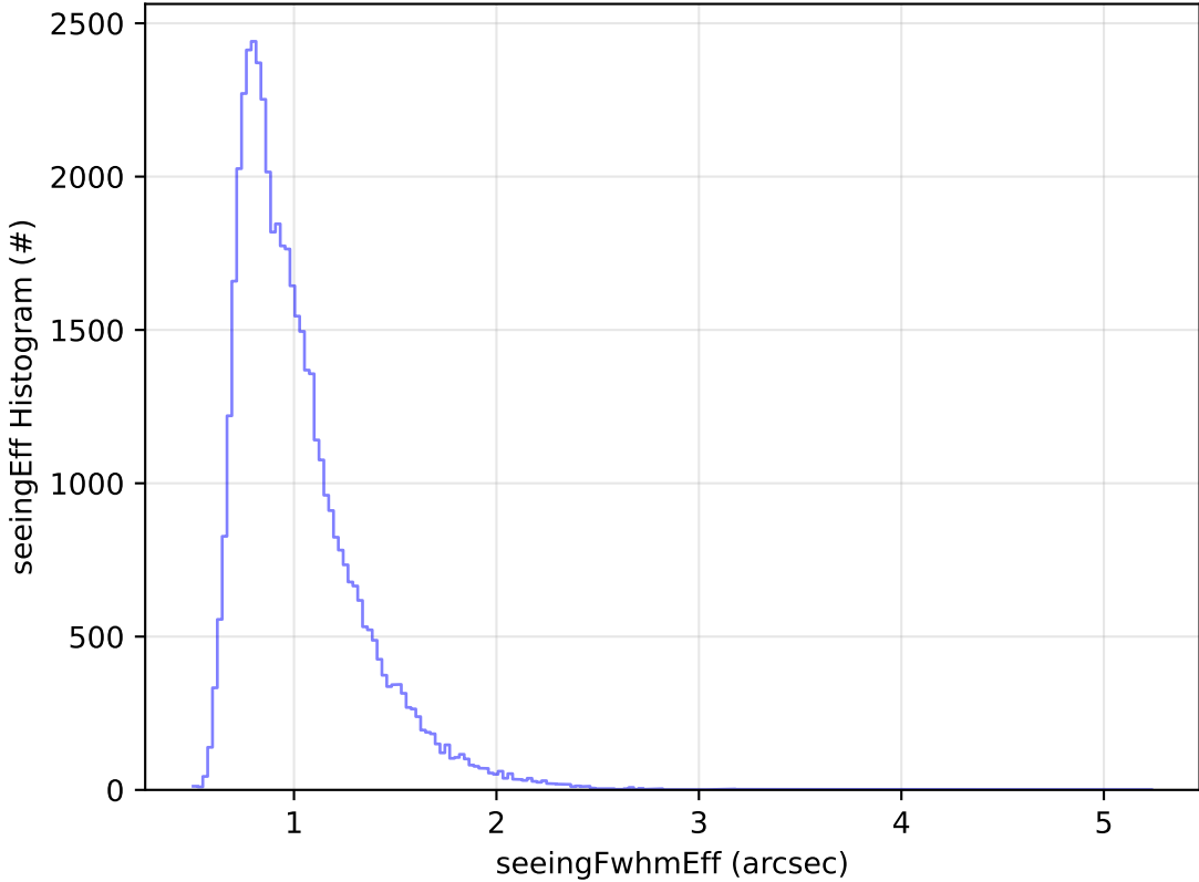
too_elab_r8_d2_giz_v3.4_10yrs Yr 1 r band: seeingEff Histogram
