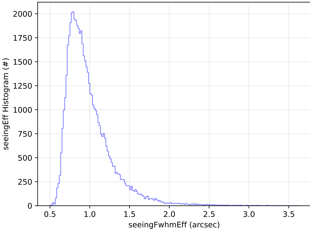
too_elab_r8_d2_giz_v3.4_10yrs Yr 1 i band: seeingEff Histogram
