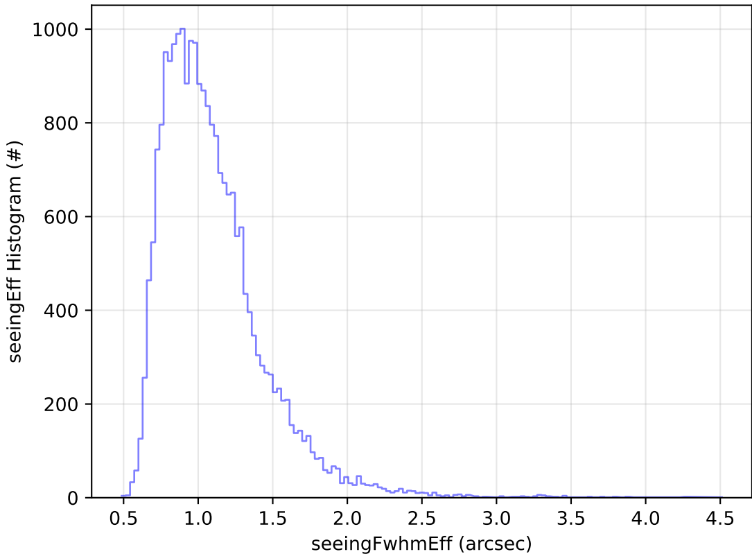
too_elab_r8_d2_giz_v3.4_10yrs Yr 1 g band: seeingEff Histogram
