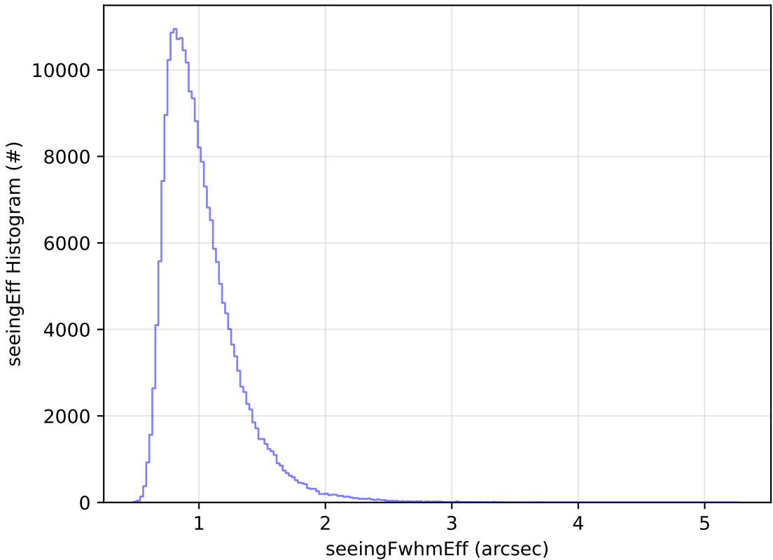
too_elab_r8_d2_giz_v3.4_10yrs Yr 1 all bands: seeingEff Histogram
