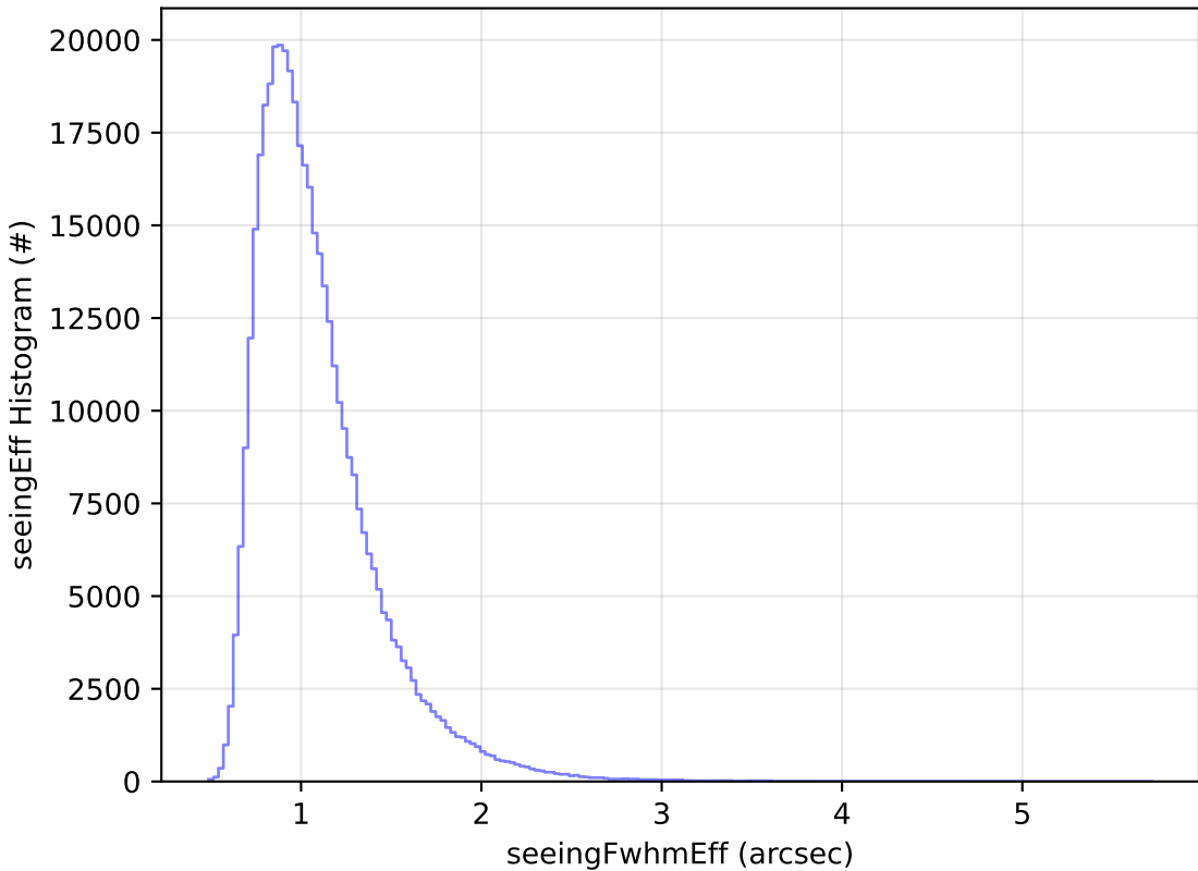
too_elab_r8_d2_giz_v3.4_10yrs WFD z band: seeingEff Histogram
